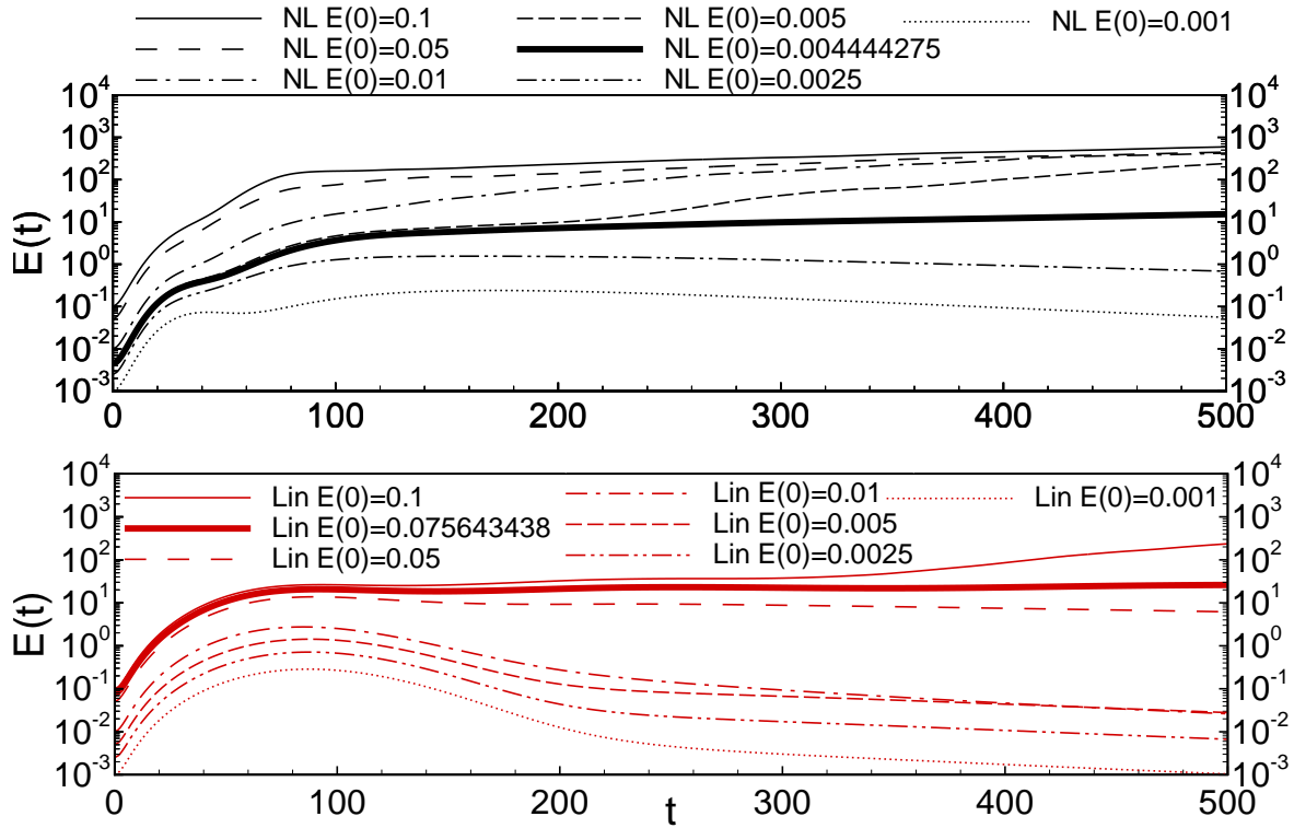
Figure 3. Evolution of the energy in time, obtained by DNS initialized with the non-linear (top frame) and linear (bottom frame) optimal perturbation for different values of the initial energy. The thick lines are the trajectories which approach saddle points on the edge of chaos.
