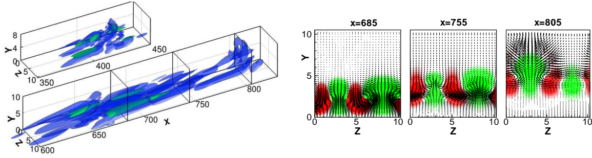
Figure 5. Snapshots of the streamwise component of the perturbation (green) and of the Q-criterion (blue) on the laminar-turbulent boundary at t = 300 and t = 700 (top and bottom frames on the left, respectively), and slices of the latter on the x = \text{constant} planes indicated in the figure (frames on the right): red and green contours indicate the positive and negative streamwise disturbance velocity, respectively; vectors represent the wall-normal and the spanwise disturbance velocity components.
