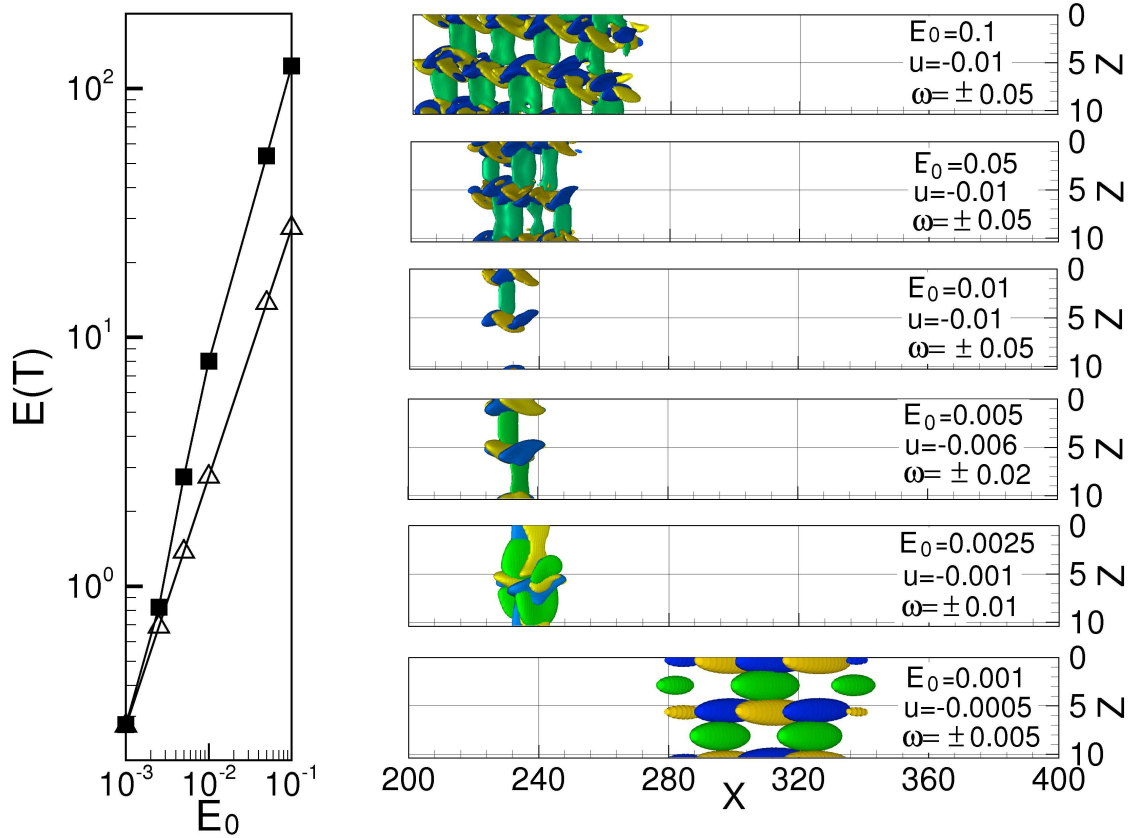
Figure 1. Optimal perturbation energy at target time T = 75 versus the initial energy E_0 obtained by a non-linear (filled squares) and a linear optimization (triangles). The initial optimal perturbations obtained by the non-linear optimization for each one of the considered initial energies (filled squares) are represented on the right, for increasing initial energy from bottom to top. Green (gray) surfaces represent negative streamwise velocity, yellow (light gray) and blue (dark gray) surfaces represent negative and positive streamwise vorticity \omega , respectively. The corresponding values are indicated in the figure.
