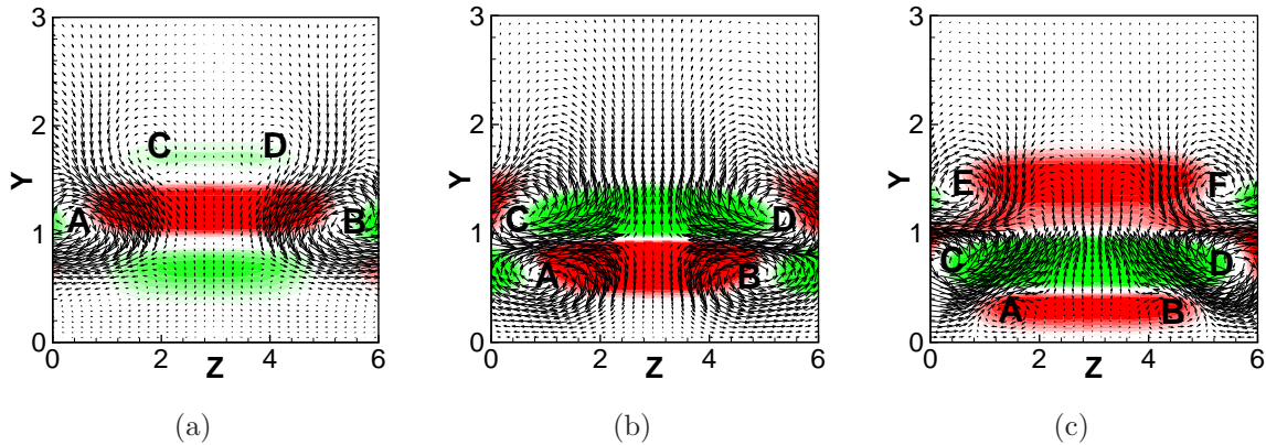
Figure 2. (Color online) Velocity components of the initial optimal perturbation obtained for Re = 610 , T = 75 , and E_0 = 0.01 , on the planes x = 224 (a), x = 228 (b), x = 232 (c). Red and green contours indicate the positive and negative streamwise disturbance velocity, respectively; vectors represent the wall-normal and the spanwise disturbance velocity components.
